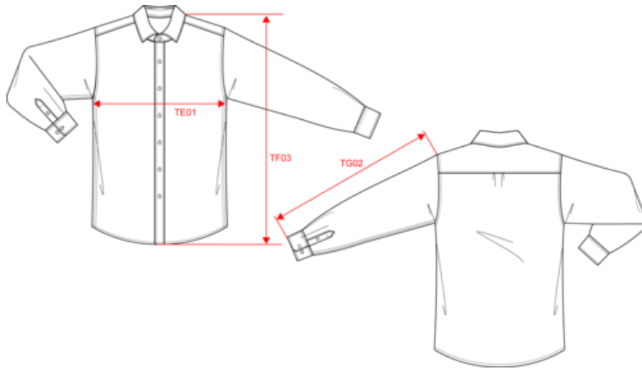
Dimensions (cm)
